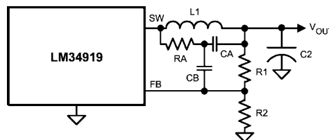
FIGURE 9. Minimum Output Ripple Using Ripple Injection
