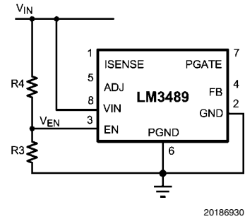
FIGURE 6. Adjustable UVLO
