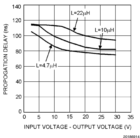
FIGURE 2. Propagation Delay
