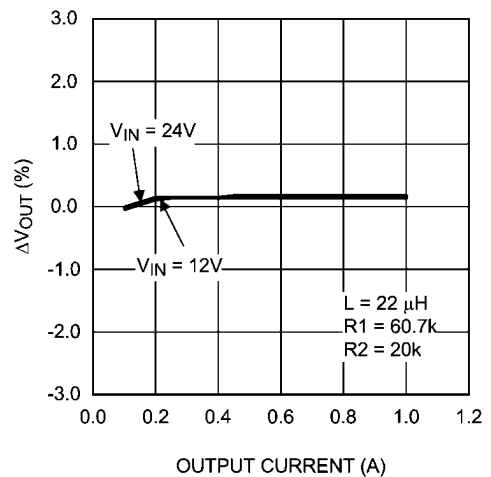
V_{OUT} Regulation vs Load Current ( V_{OUT} = 5V , L = 22\mu\text{H} )
