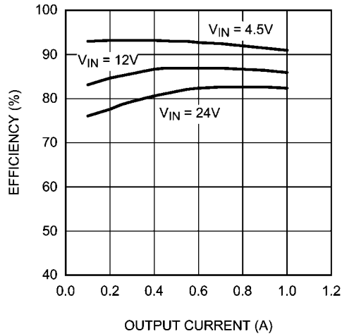
Efficiency vs Load Current ( V_{OUT} = 3.3V , L = 22\mu\text{H} )
