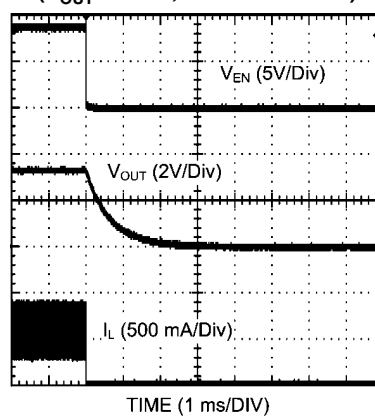
Shutdown Transient ( V_{OUT} = 3.3V , 500 mA Loaded)
