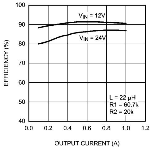
Efficiency vs Load Current ( V_{OUT} = 5V , L = 22\mu\text{H} )
