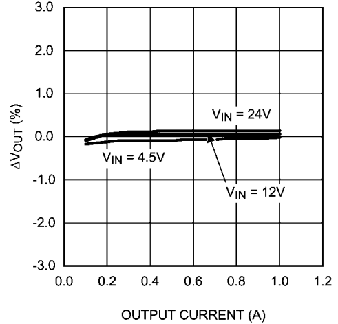
V_{OUT} Regulation vs Load Current ( V_{OUT} = 3.3V , L = 22\mu\text{H} )
