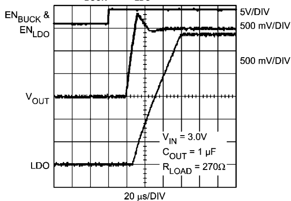
LDO Turn ON ( EN_{BUCK} = EN_{LDO} = Low to High)
