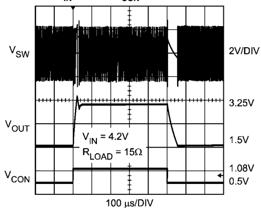
V_{CON} Voltage Response ( V_{IN} = 4.2V , V_{CON} = 0.5V / 1.1V )
