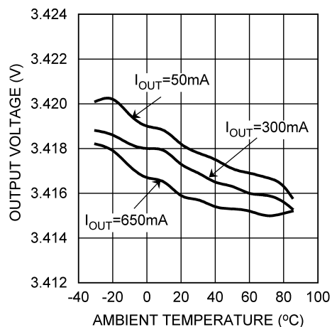
Output Voltage vs Temperature ( V_{IN} = 4.2V , V_{OUT} = 3.4V )
