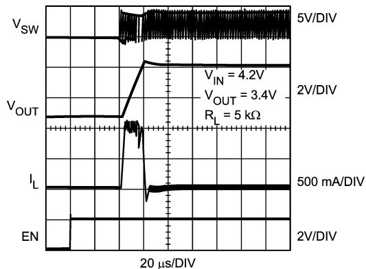
Startup ( V_{IN} = 4.2V , V_{OUT} = 3.4V , R_{LOAD} = 5k\Omega )
