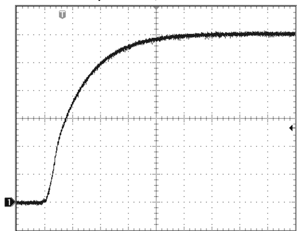
Startup Behavior, Load = 150mA
