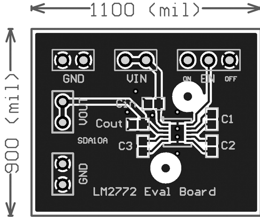
FIGURE 1. Top Layer
