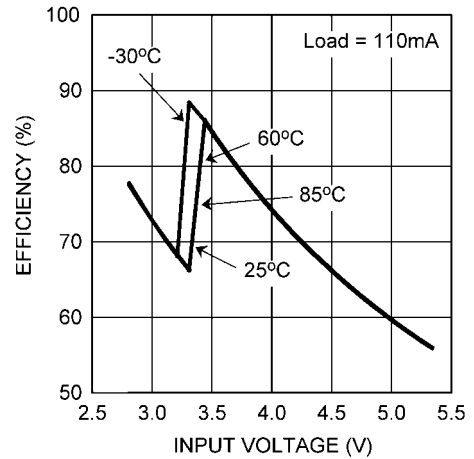
Efficiency vs. Input Voltage, 4.5V Mode
