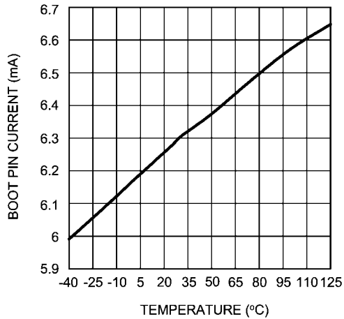
BOOT Pin Current vs Temperature for BOOT Voltage = 5V F_{SW} = 300\text{kHz} , FDS6898A FET, No-Load
