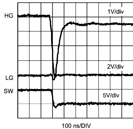
Switch Waveforms (HG Falling) V_{CC} = 3.3\text{V} , V_{IN} = 5\text{V} , V_{REF} = 0.6\text{V} , V_{OUT} = 1.2\text{V} I_{OUT} = 4\text{A} , C_{SS} = 12\text{nF} , F_{SW} = 300\text{kHz}
