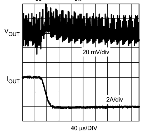
Load Transient Response ( I_{OUT} = 4A to 0A ) V_{CC} = 3.3V , V_{IN} = 5V , V_{REF} = 0.6V , V_{OUT} = 1.2V C_{SS} = 12nF , F_{SW} = 300kHz
