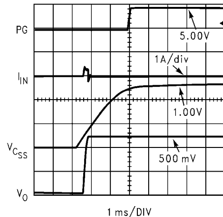
Start-Up (No-Load)
