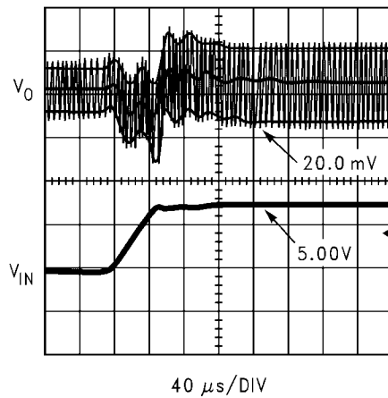
Line Transient Response ( V_{IN} = 5V to 12V) V_O = 1.2V , I_O = 5A F_{SW} = 300kHz
