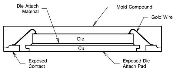
FIGURE 8. Internal LLP Connection
