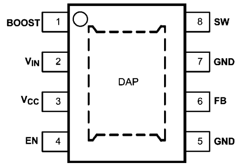
8-Pin eMSOP - TOP VIEW NS Package Number MUY08A
