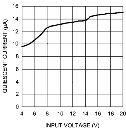
Shutdown I_Q vs. Input Voltage
