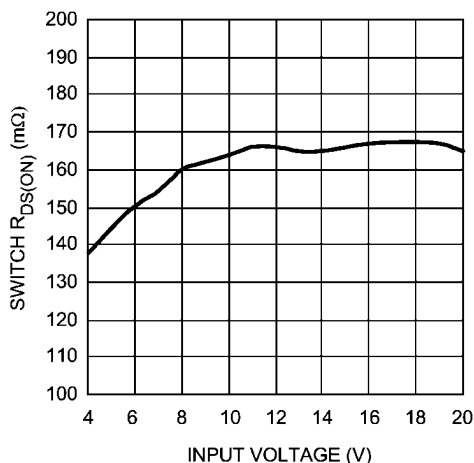
Buck 2 R_{DS(ON)} vs. Input Voltage
