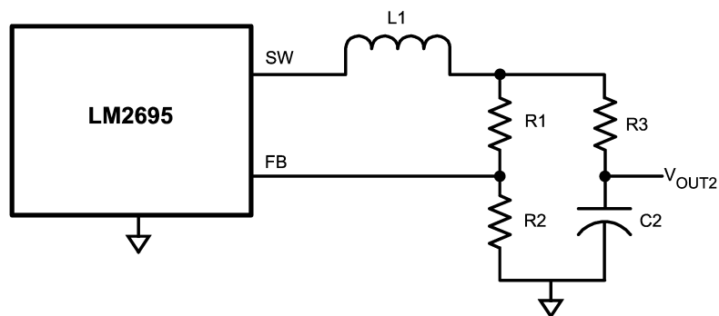
FIGURE 4. Low Ripple Output Configuration
