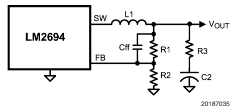
FIGURE 17. Low Output Ripple Using a Feedforward Capacitor
