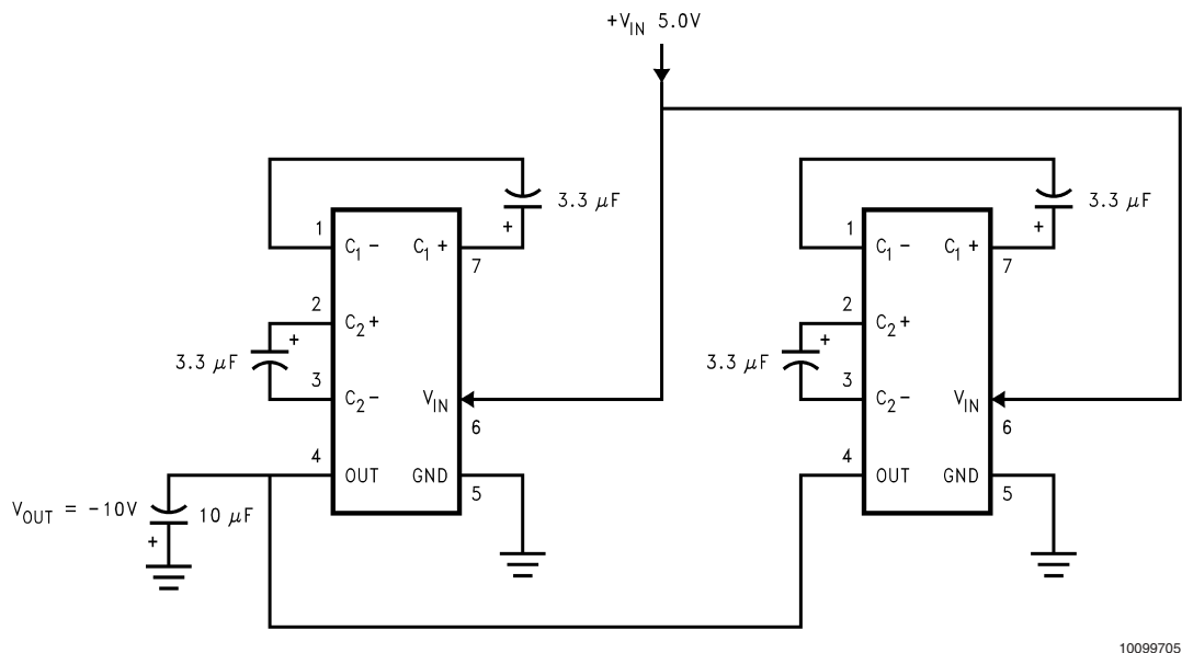
FIGURE 3. Paralleling Devices
