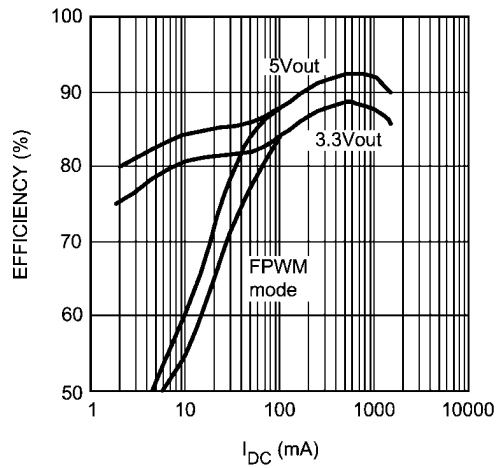
Efficiency vs Load Current (330kHz)
