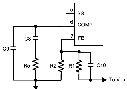
FIGURE 10. Compensation Network
