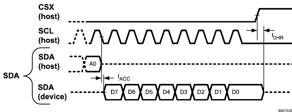
FIGURE 5. SPI Interface
