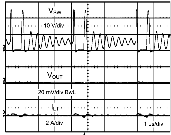
FIGURE 10. Discontinuous Operation using Diode Emulation Mode at 24V IN with JMP1 Installed
