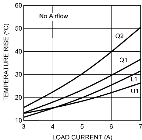
FIGURE 3. Temperature Rise at 24V IN with 6 μH Cooper Inductor
