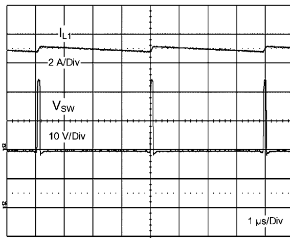
FIGURE 5. Short Circuit at 24V IN Room Temperature
