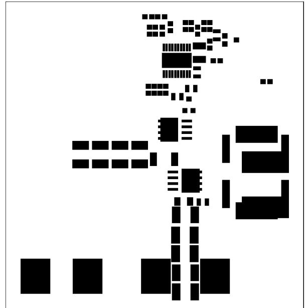
TOP SOLDER PASTE MASK (.CRS) AS VIEWED FROM TOP 881013161-001
