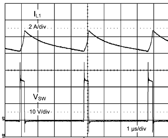
FIGURE 6. Short Circuit at 24V IN 125°C
