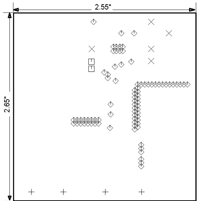
DRILLS AND DIMENSIONS (.FAB) LAYER AS VIEWED FROM TOP 880013161-001
