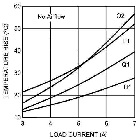
FIGURE 4. Temperature Rise at 24V IN with 5.6 μH Pulse Inductor
