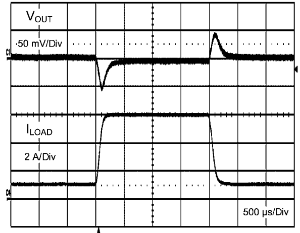
FIGURE 11. Transient Response at 24V IN
