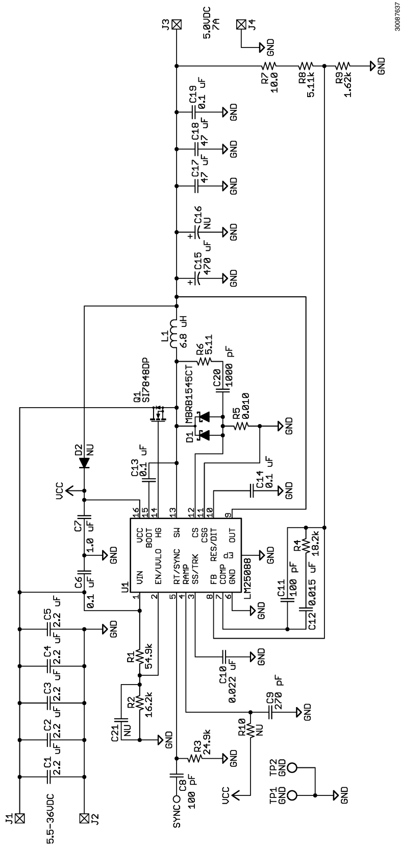
FIGURE 14. LM25088-1 Application Schematic
