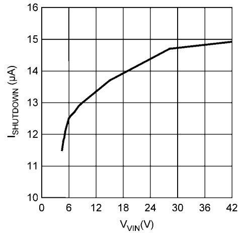
Shutdown Current
