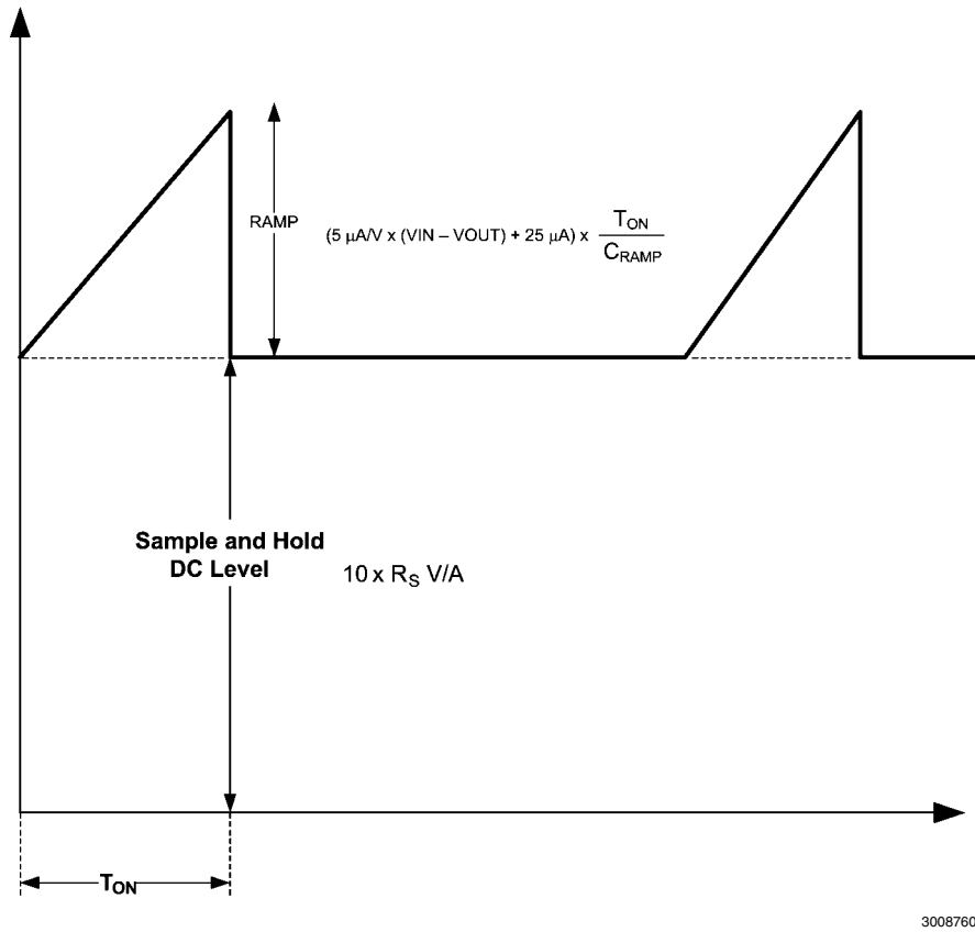
FIGURE 3. Composition of Current Sense Signal
