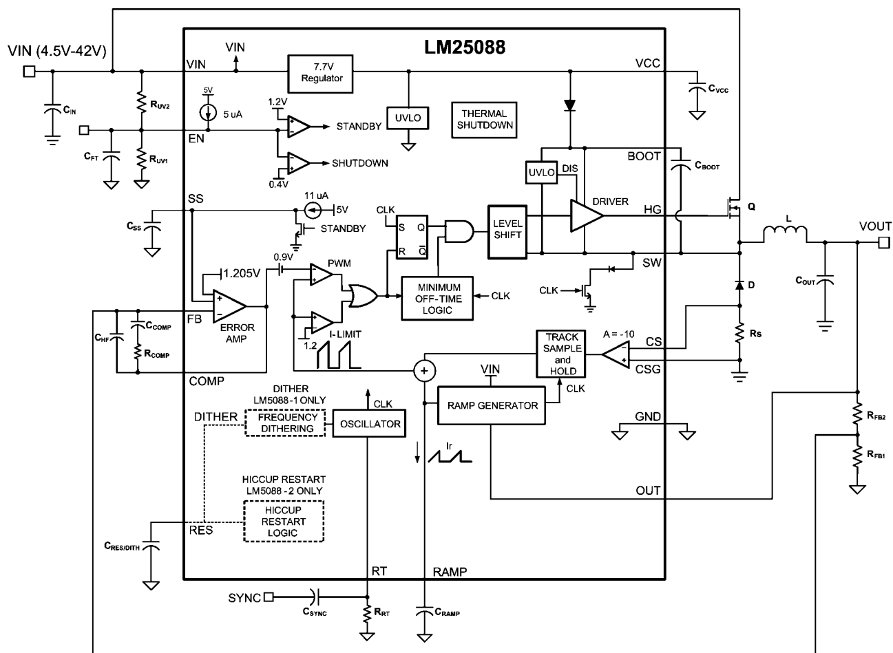
FIGURE 1. Block Diagram
