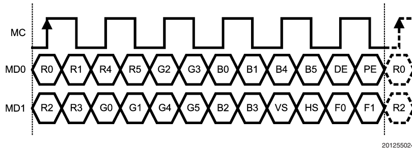
FIGURE 9. 18-bit RGB Display Mode Transaction
