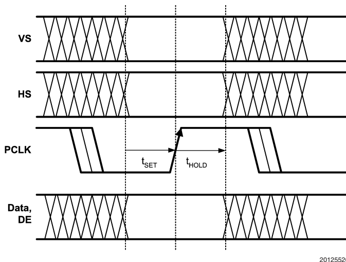
FIGURE 11. Serializer Mode Input Timing for RGB Interface
