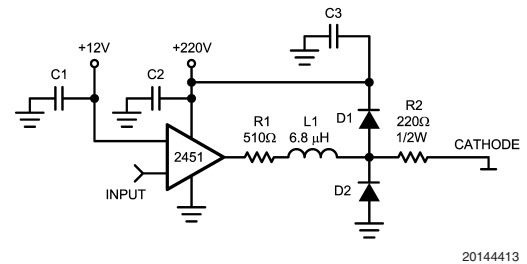
FIGURE 13. One Channel of the LM2451 with the Recommended Application Circuit
