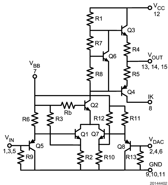
FIGURE 2. Simplified Schematic Diagram (One Channel)
