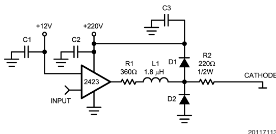
FIGURE 13. One Channel of the LM2423 with the Recommended Application Circuit
