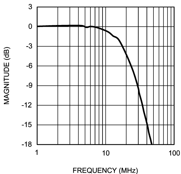
FIGURE 6. Bandwidth
