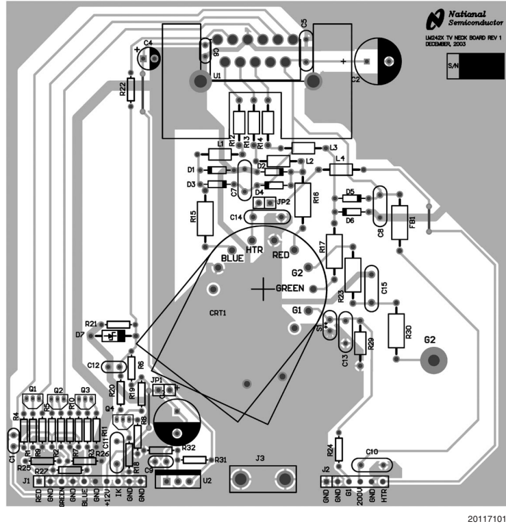
FIGURE 15. LM2423 DTV Demonstration Board Layout
