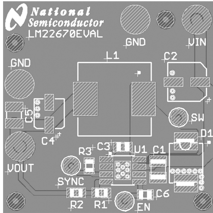
FIGURE 6. Top Layer
