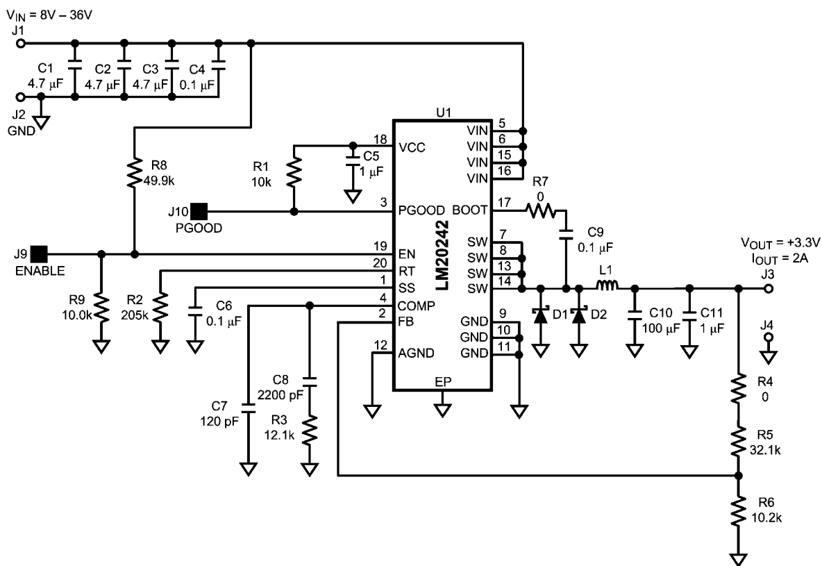
FIGURE 10. Typical Application Schematic
