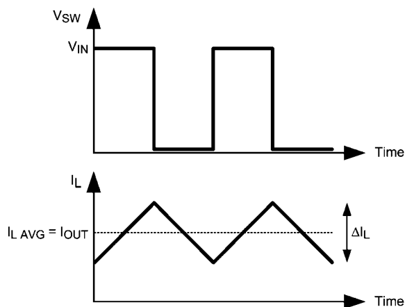
FIGURE 3. Switch and Inductor Current Waveforms
