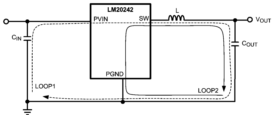
FIGURE 9. Schematic of LM20242 Highlighting Layout Sensitive Nodes
