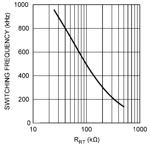
Oscillator Frequency vs. R_{RT}
