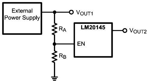
FIGURE 6. Sequencing LM20145 with Precision Enable
