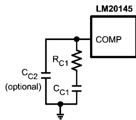
FIGURE 5. Compensation Network for LM20145
