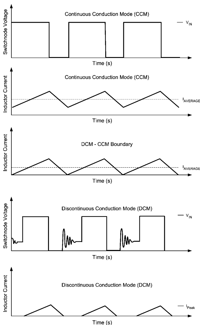
FIGURE 1. Modes of Operation for LM20145
