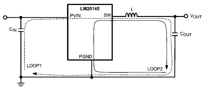
FIGURE 10. Schematic of LM20145 Highlighting Layout Sensitive Nodes
