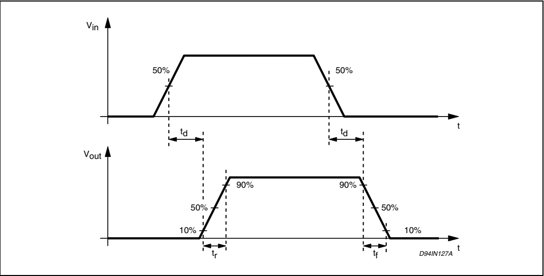
Figure 4. Switching waveforms
