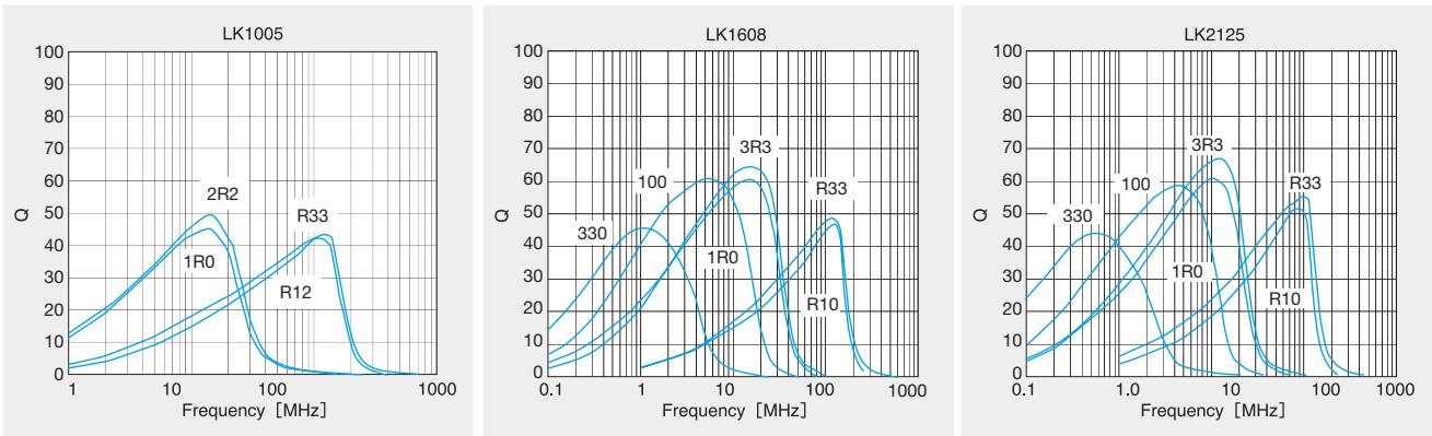
Q-周波数特性例 Q-vs-Frequency characteristics (Measured by HP4294A or HP4291A)
