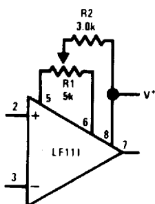
Offset Balancing
