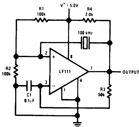
Crystal Oscillator
