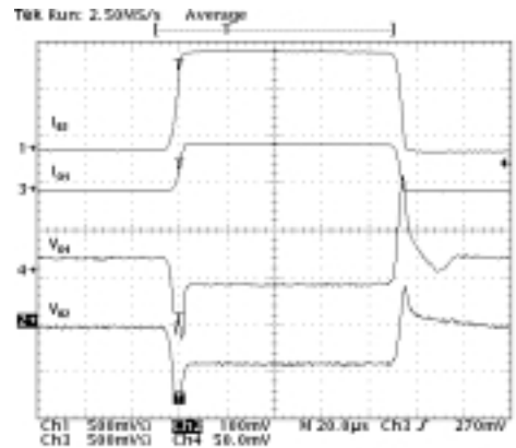
Figure 25: Load Transient
