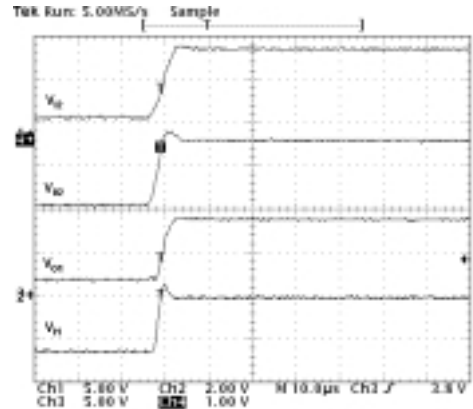
Figure 27: Start up Transient V_{O1}
