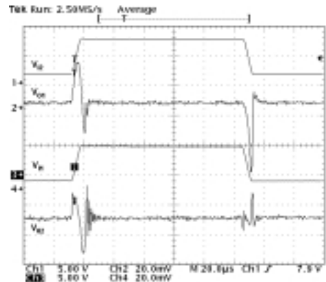
Figure 26: Line Transient V_{O1,2}
