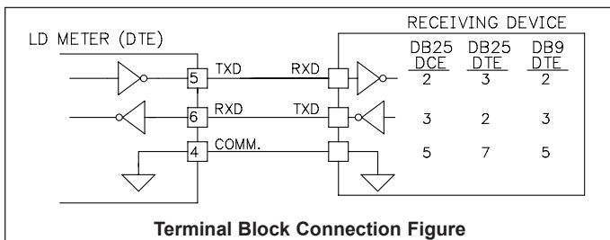
Terminal Block Connection Figure
