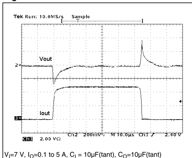
Figure 26. Load transient
