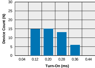
LBA120 - FormB Typical Turn-On Time (N=50 Ambient Temperature = 25°C) (Load Current = 170mADC; I_F = 5mADC)
