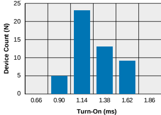
LBA120 - FormA Typical Turn-On Time (N=50 Ambient Temperature = 25°C) (Load Current = 170mADC; I_F = 5mADC)
