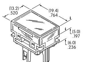
AT4163 Rectangular
