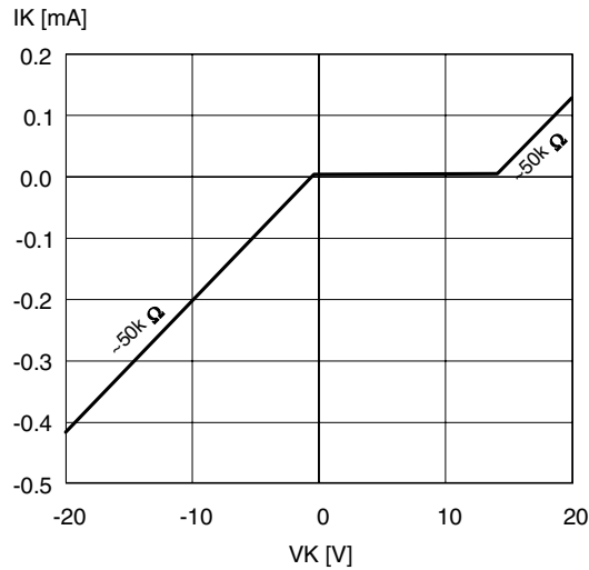
Figure 6. I(V) characteristics of the K-Line for TX = HIGH and VVS=13.5V
