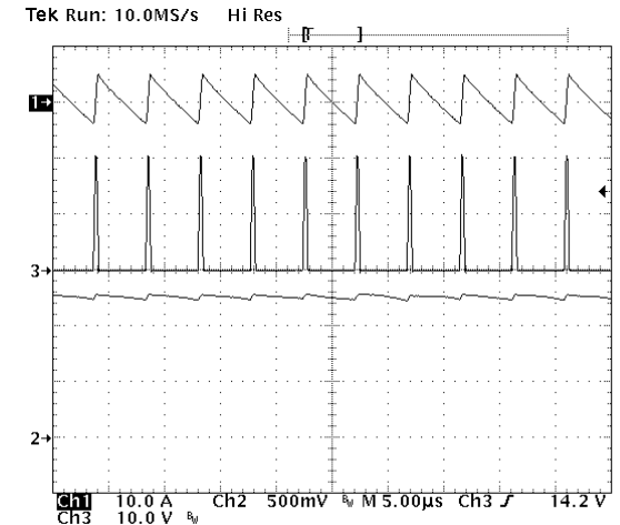
Figure 22. Normal functionality in PWM mode.
