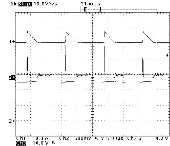
Figure 21. Normal functionality in PSK mode.
