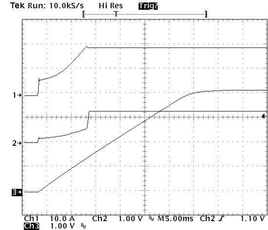
Figure 20. Soft Start with 20A load.
