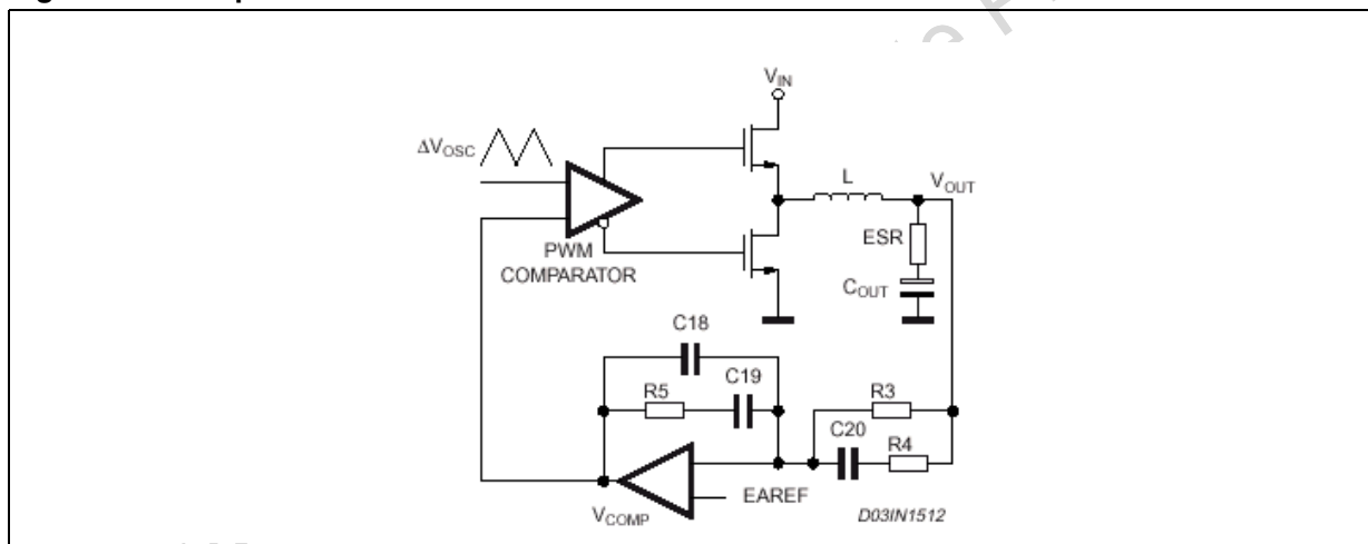
Figure 11. Compensation Network
