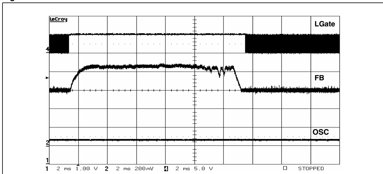
Figure 12. OVP not latched
