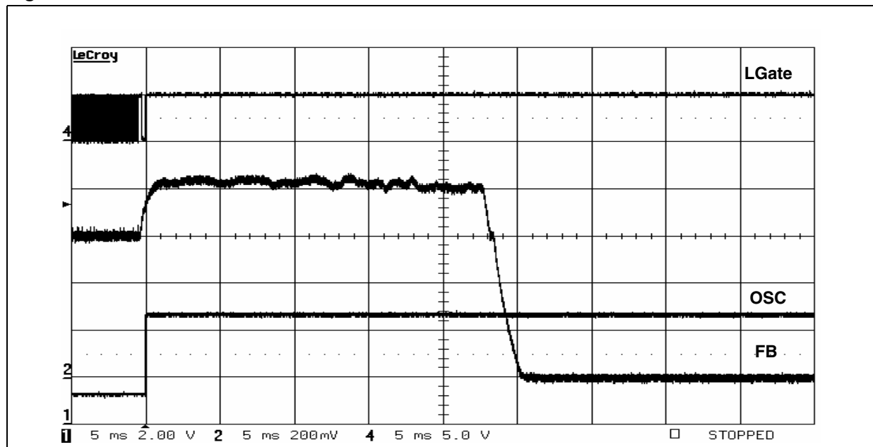
Figure 13. OVP latched
