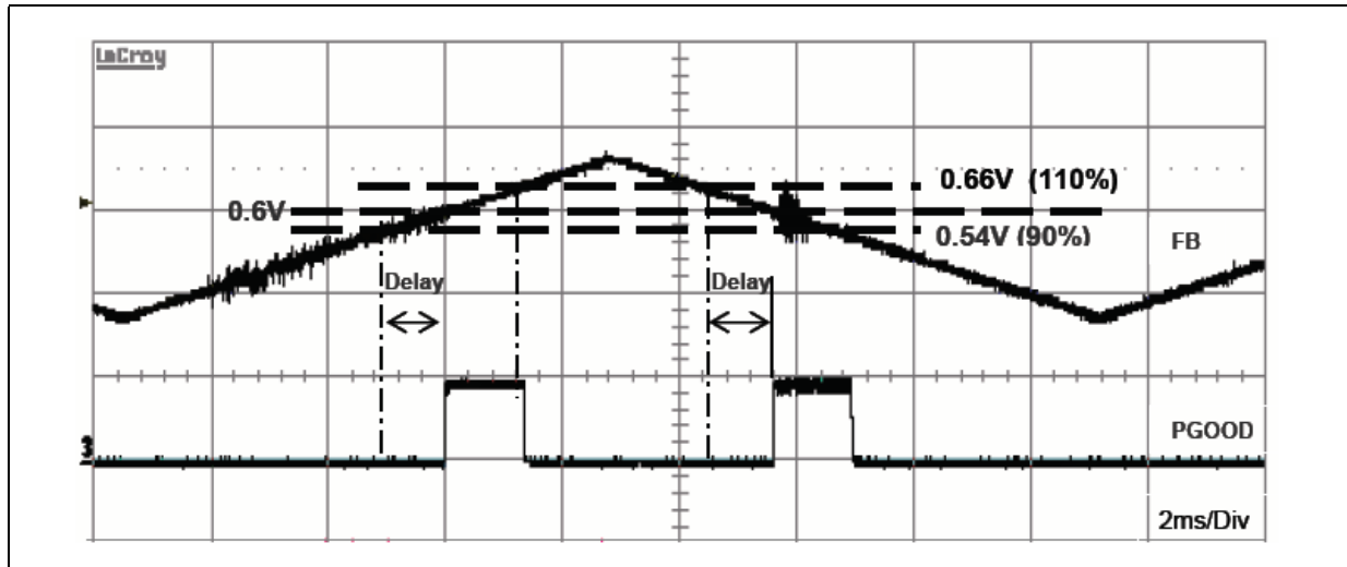
Figure 11. PGOOD signal
