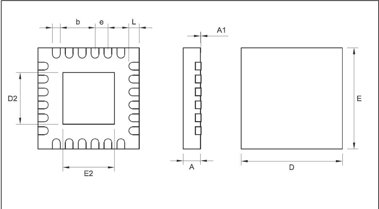
Figure 43. Package dimensions
