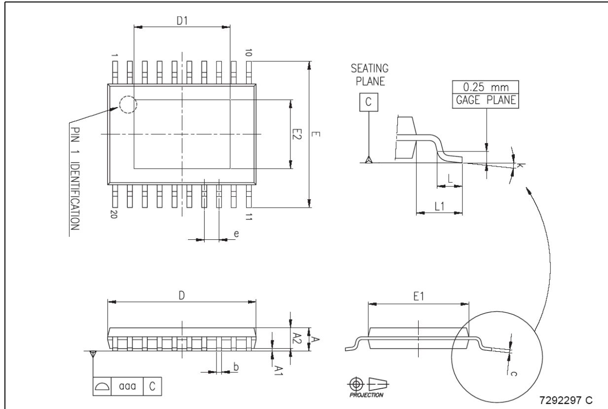
Figure 42. Package dimensions
