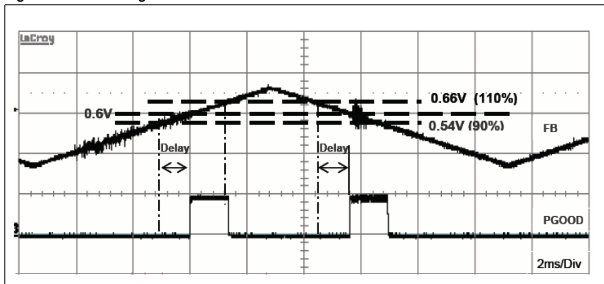
Figure 13. PGOOD signal
