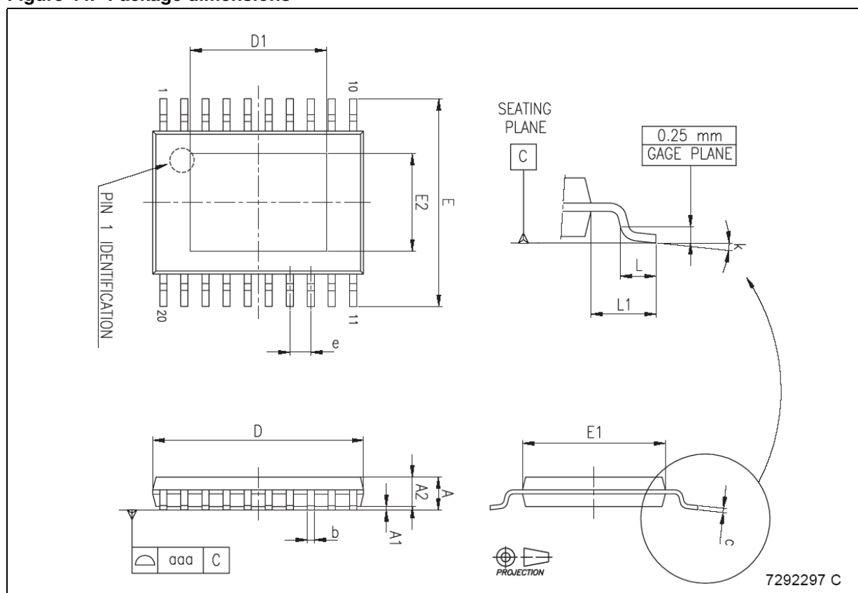
Figure 44. Package dimensions
