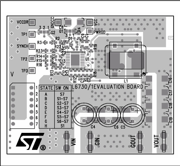
Figure 32. Top layer
