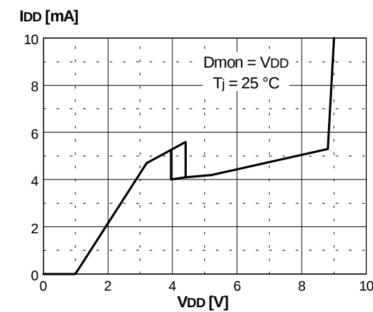
Figure 2. IC Supply current vs. supply voltage
