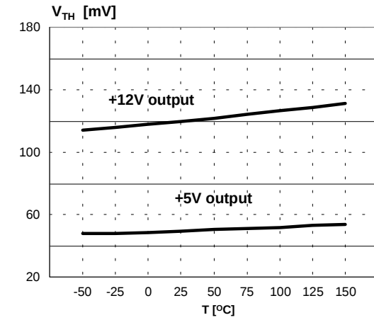
Figure 5. Output's current sense thresholds
