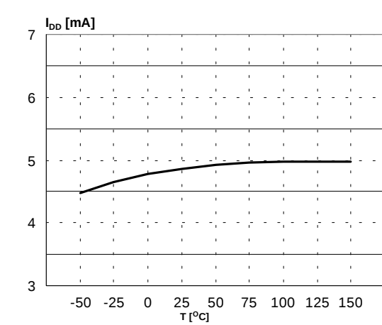
Figure 3. IC Supply current
