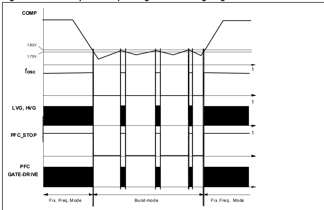
Figure 8. Load-dependent operating modes: timing diagram
