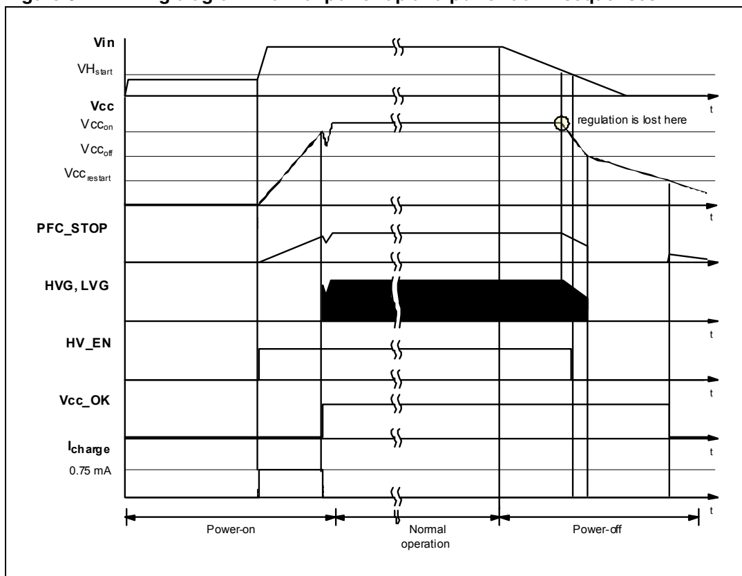
Figure 6. Timing diagram: normal power-up and power-down sequences
