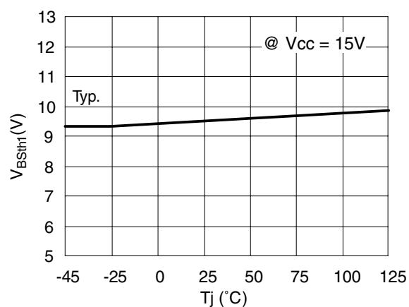
Figure 9. V_{BOOT} UV Turn On Threshold vs. Temperature
