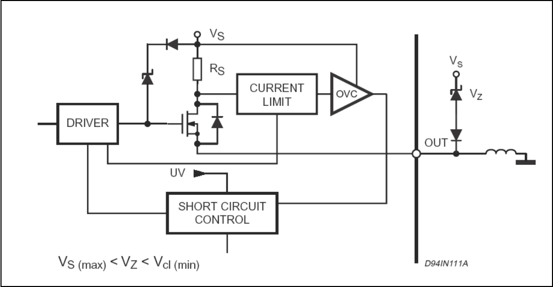
Figure 8. Application schematic
