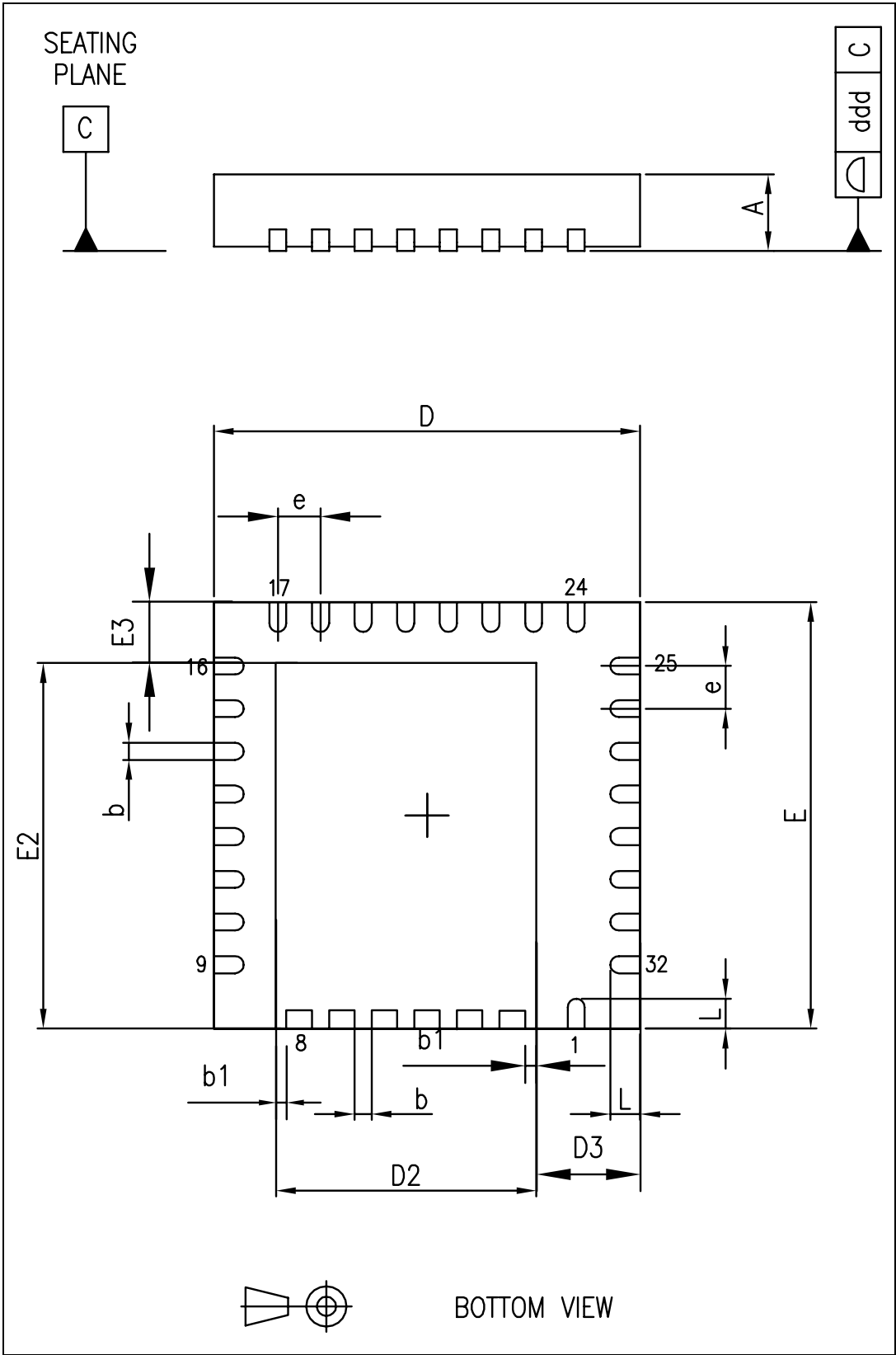
Figure 18. Package dimensions
