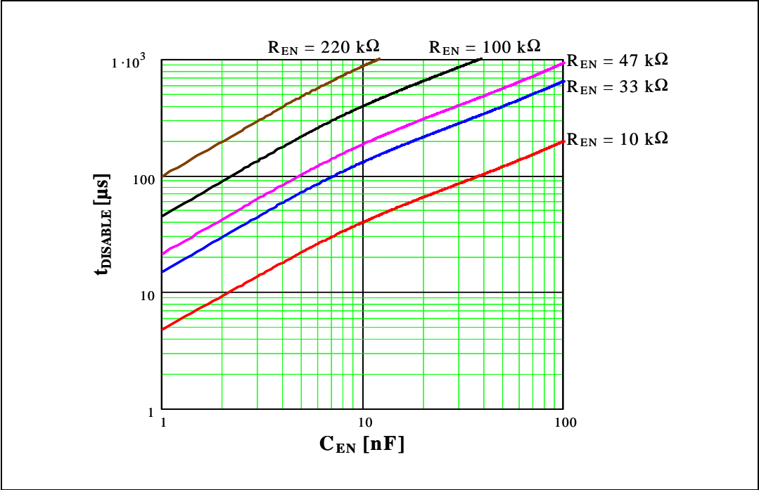
Figure 10. t_{\text{DISABLE}} versus C_{\text{EN}} and R_{\text{EN}} ( V_{\text{DD}} = 5 \text{ V} )
