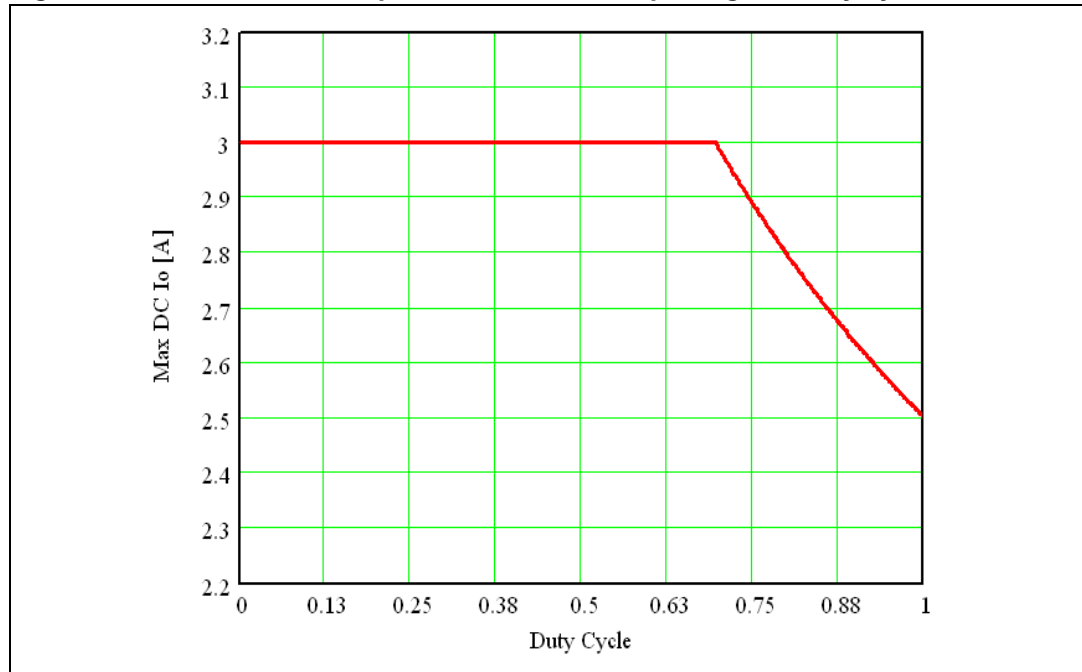
Figure 8. Maximum DC output current for VQFN package vs duty cycle
