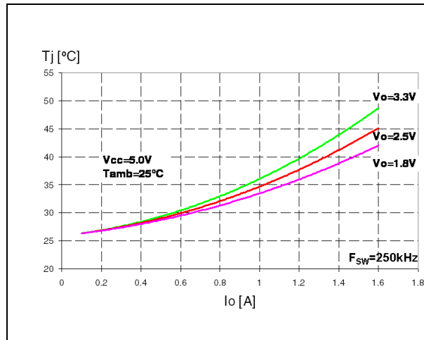
Figure 24. Junction temperature vs output current
