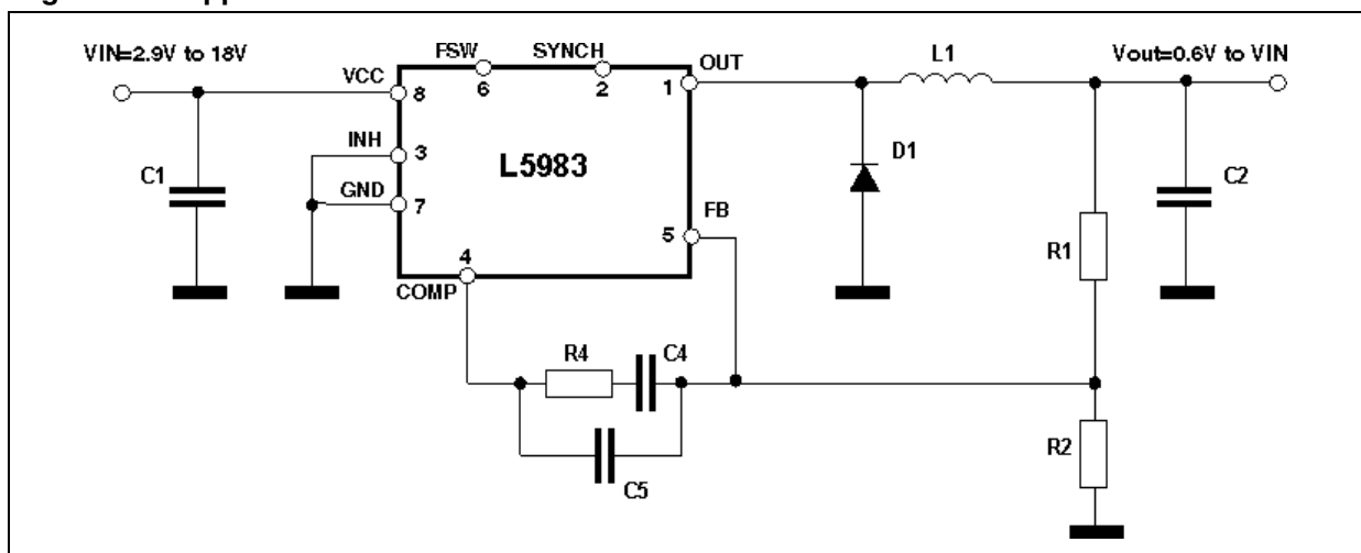
Figure 1. Application circuit
