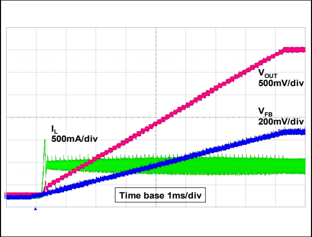
Figure 32. Soft-start
