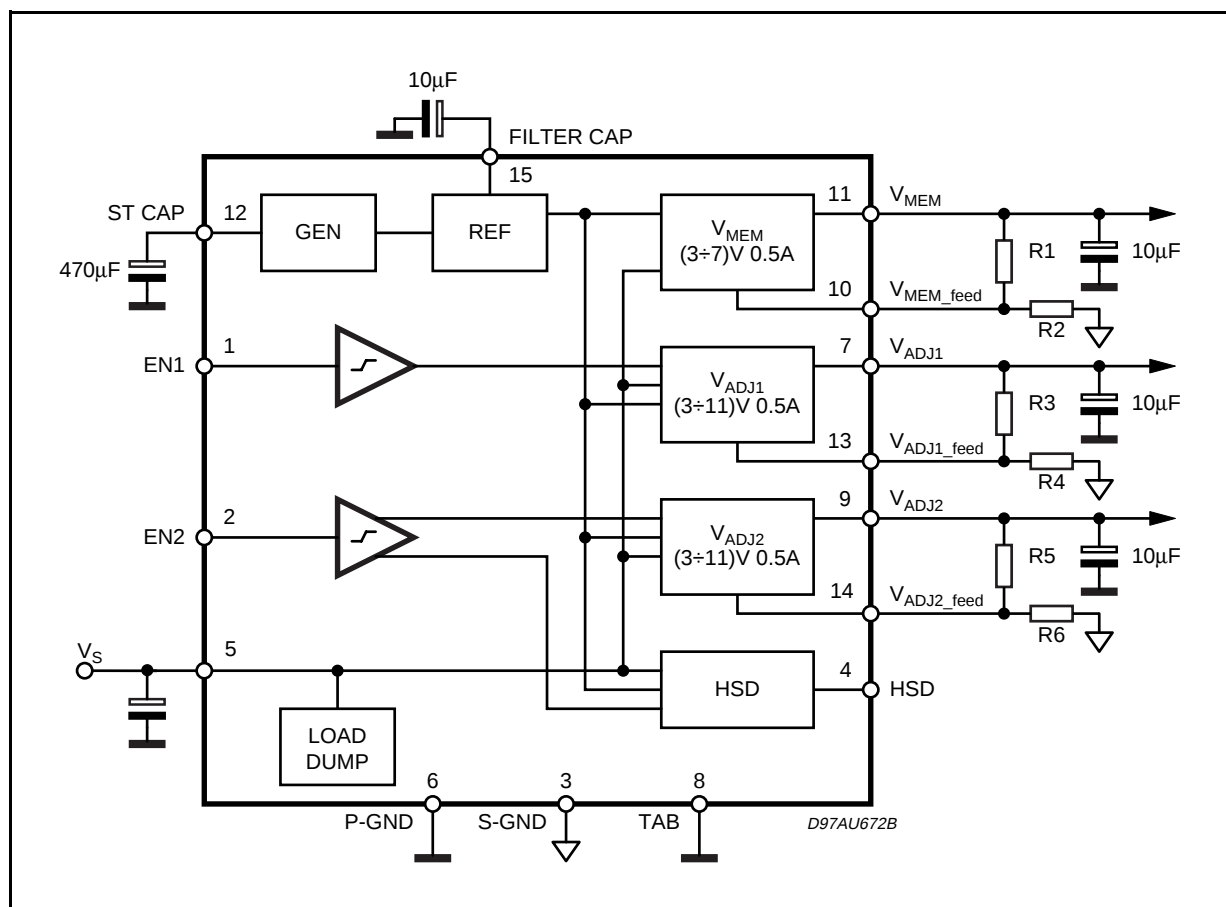
Figure 1. Application circuit.
