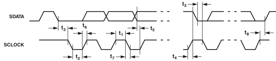
Figure 1. MPU Port Timing Diagram
