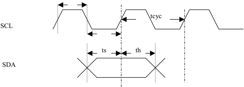
Figure 2. EEPROM Input Timing Diagram
