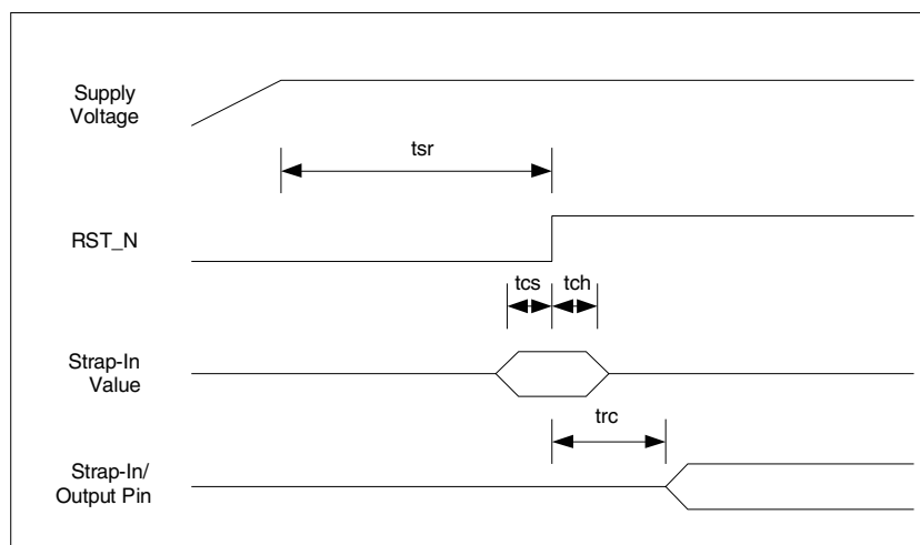
Figure 23. Reset Timing
