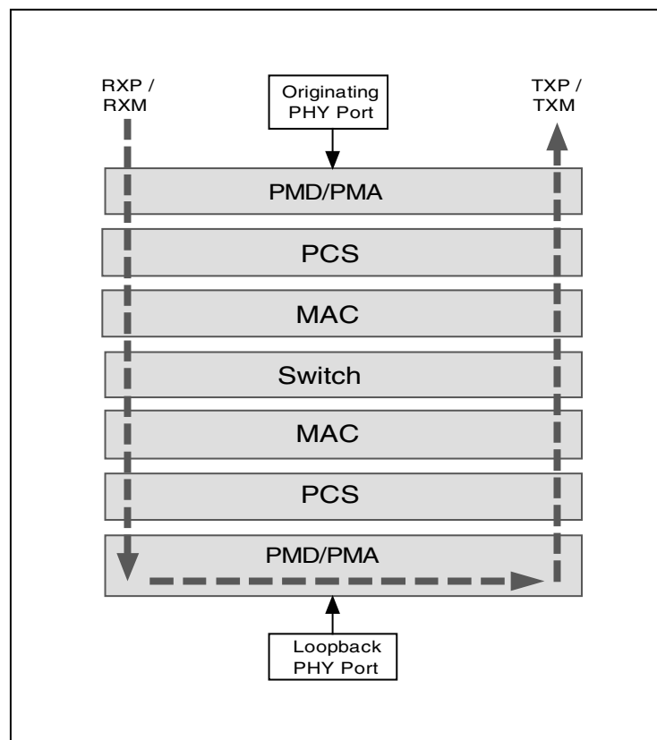
Figure 12. Loopback Path
