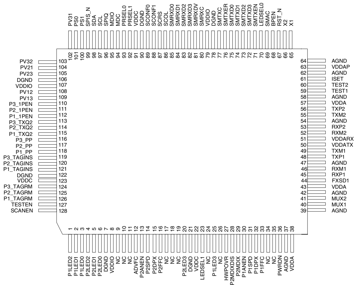
128-Pin PQFP (Top View)
