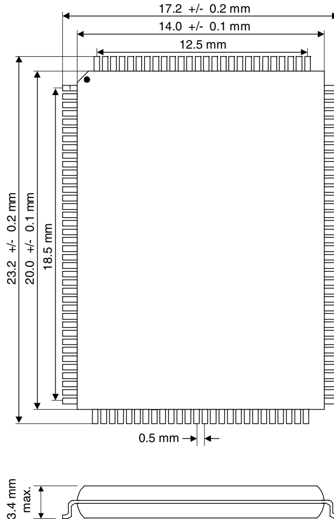
128-Pin PQFP Package
