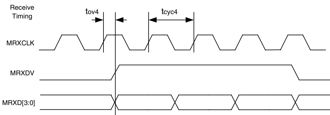
Figure 18. MAC-Mode MII Timing – Data Input to MII
